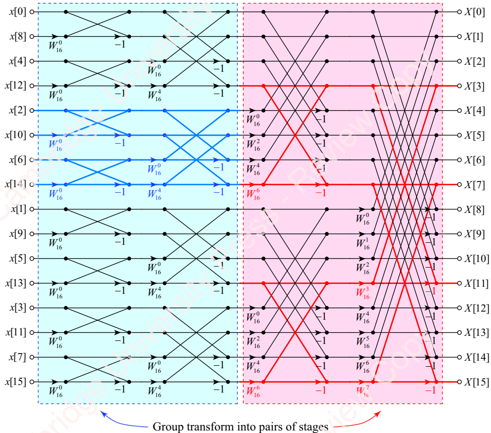
Figure 11.17 Understanding a radix-4 transform in terms of two radix-2 transforms
